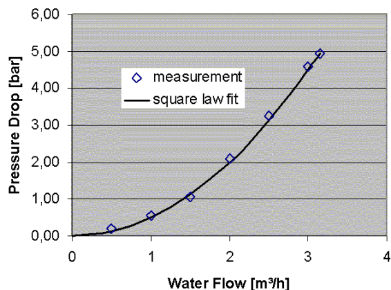
Pressure Drop
