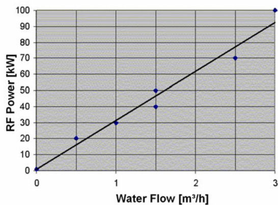
RF Power and Water Flow for 100°C Surface Temperature
